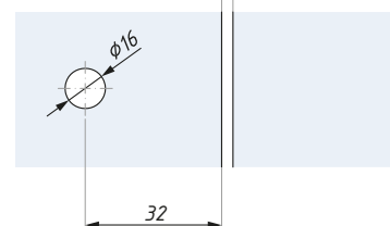
GK625 Zaczepek GK625 Strike
